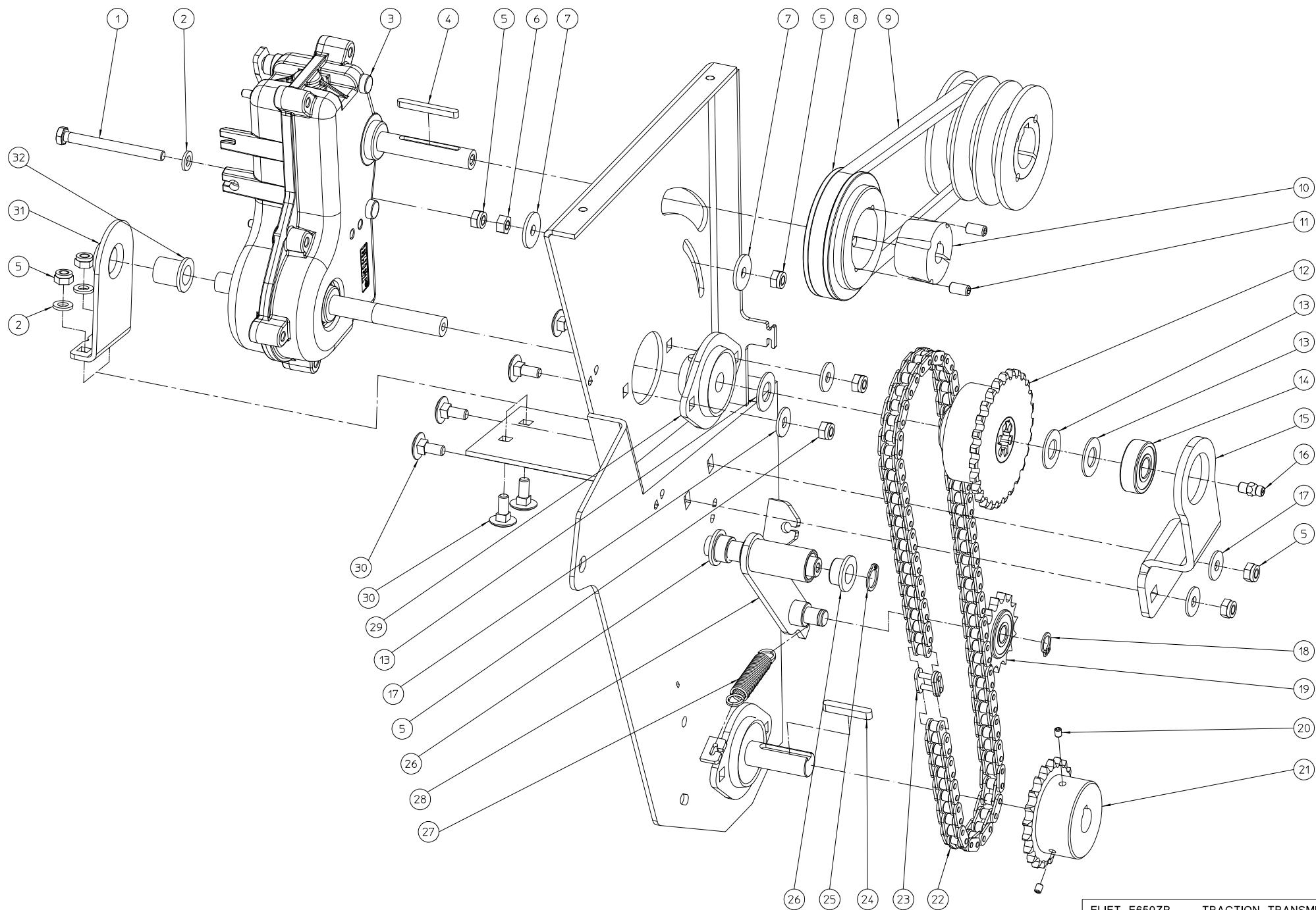
ELIET E650ZR --- TRACTION TRANSMISSION
