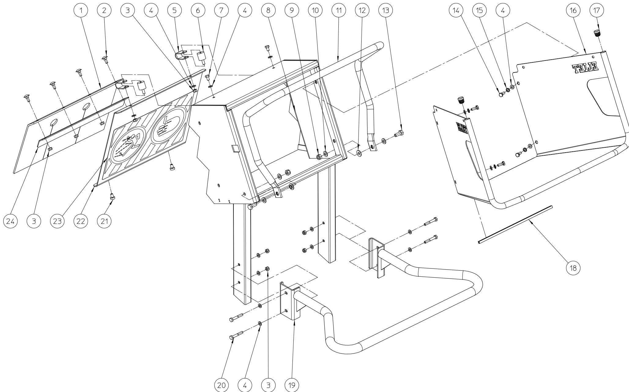
ELIET MAJOR 4S -- MACHINE FRONT SIDE
