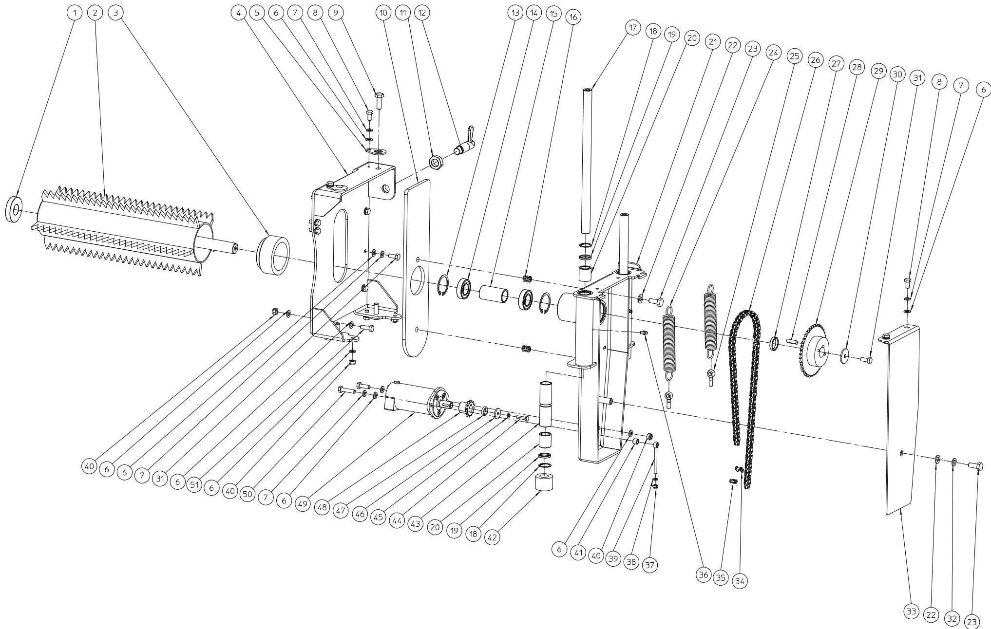
ELIET PROF6 - IN FEED ROLLER
